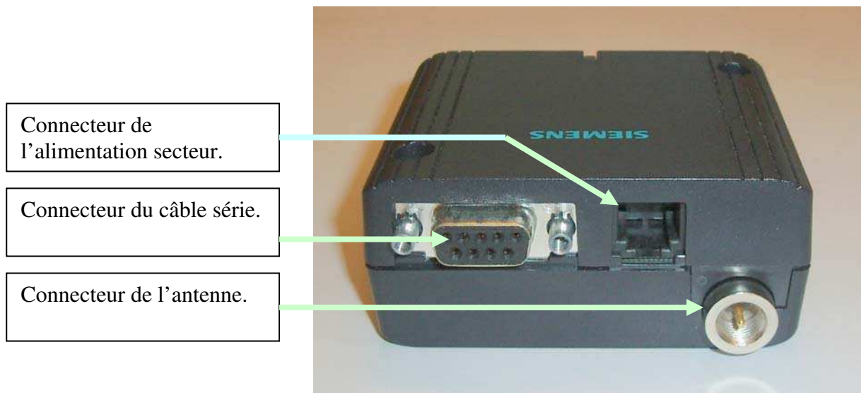
Figure 5. Modem GSM
